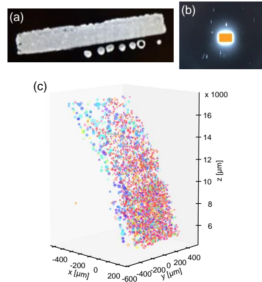
Figure 2. (a) a slice from the tomography imaging at SPring-8. The balls under the aluminium sample are glass beads that make it easier to identify positions in the samples. (b) the DCT data where every bright spot around the centre is a diffraction-projected grain image with a certain orientation. (c) the 3DXRD result image where every circle represents a grain. The diameter and colour of the circles corresponds to the grain size and orientation, respectively.
